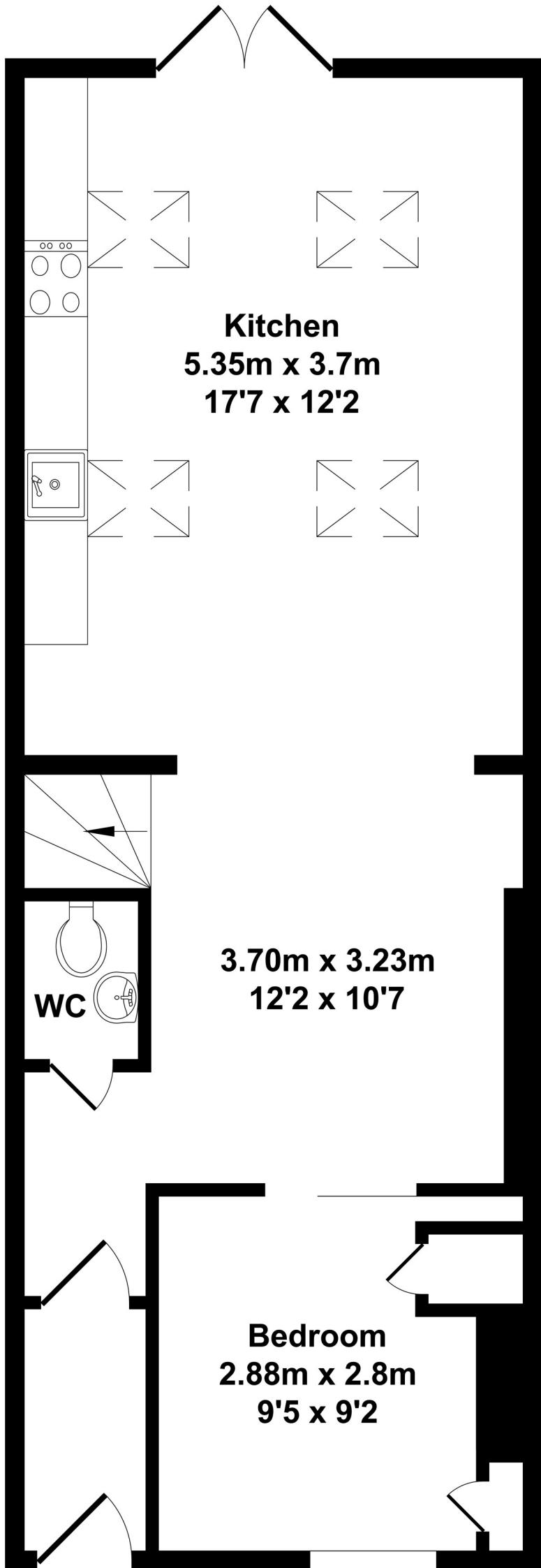
Ground Floor Approx. Floor Area 45.82 Sq.M. (493 Sq.Ft.)
